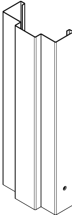
Countersink Anchor shown in 18 ga. galvanneal steel
