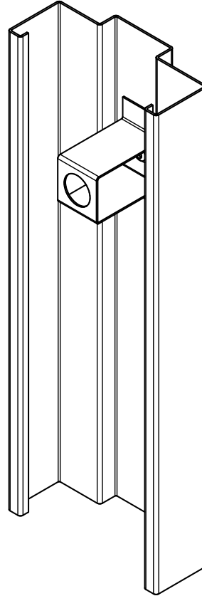
EWA Hat Style shown welded in 18 ga. galvanneal steel
